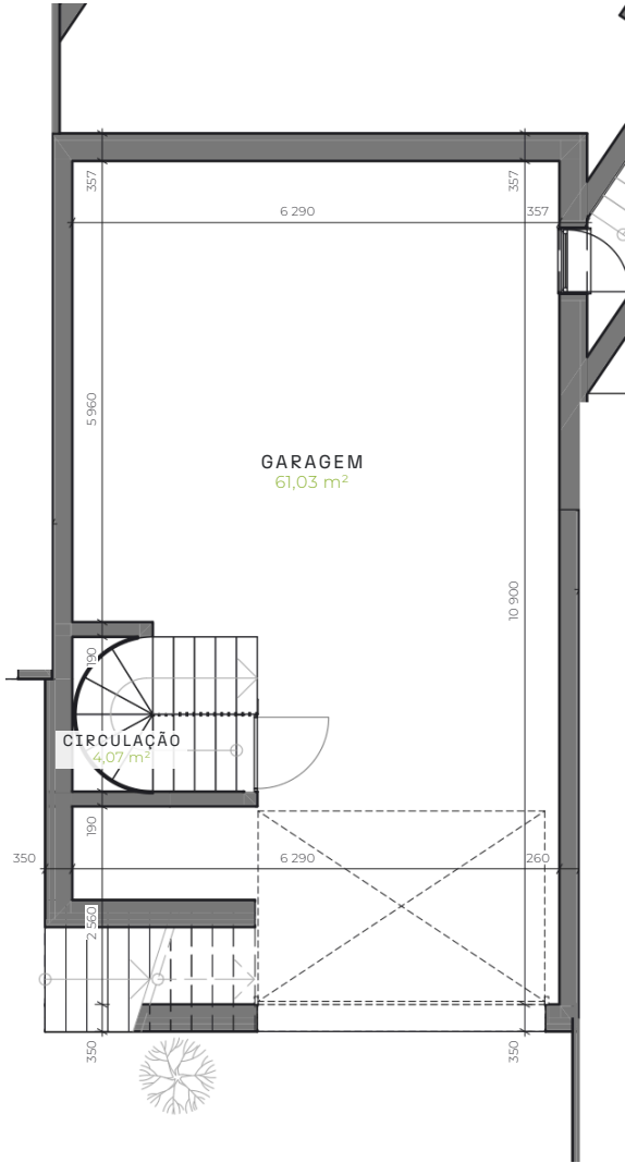
CAVE BASEMENT · 79,92 M²
